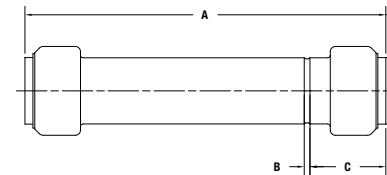
Slip Coupling
