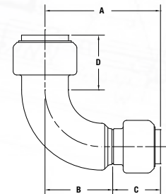
Elbow 90 Reducing
