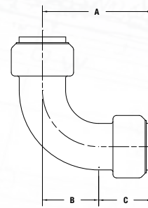
Elbow 90
